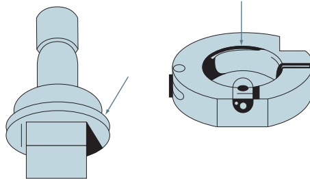
Punch with reinforced shoulder and alignment ring with large inside diameter
